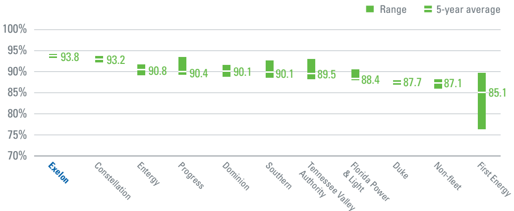
RANGE OF 5-YEAR FLEET CAPACITY FACTOR, 2004-2008
